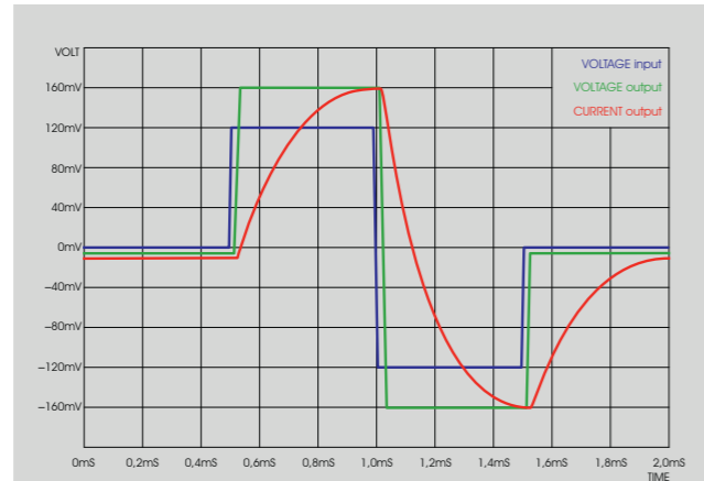
Fig. 1: Voltage amplifier simulation
